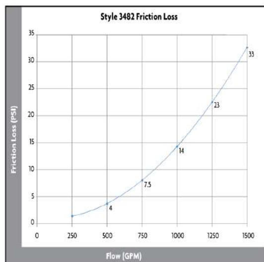
3482 Friction Loss
